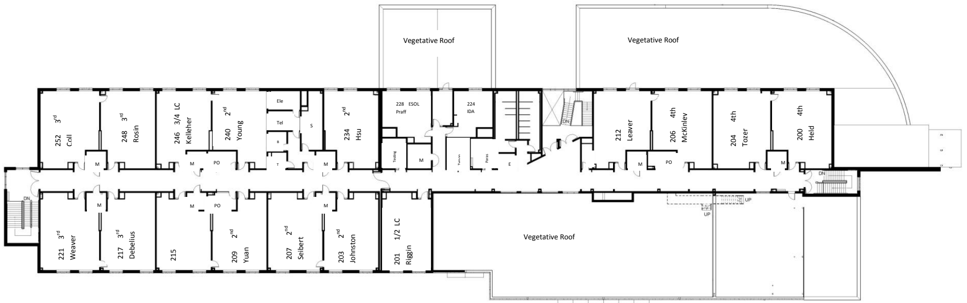
UPPER LEVEL FLOOR PLAN
